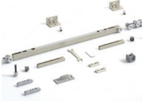
60KG SLIDING FOLDING DOOR SYSTEM SDS-ALB-S5-001
